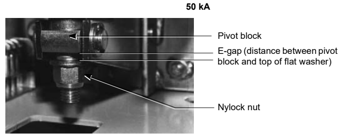
Figure 23: E-gap
